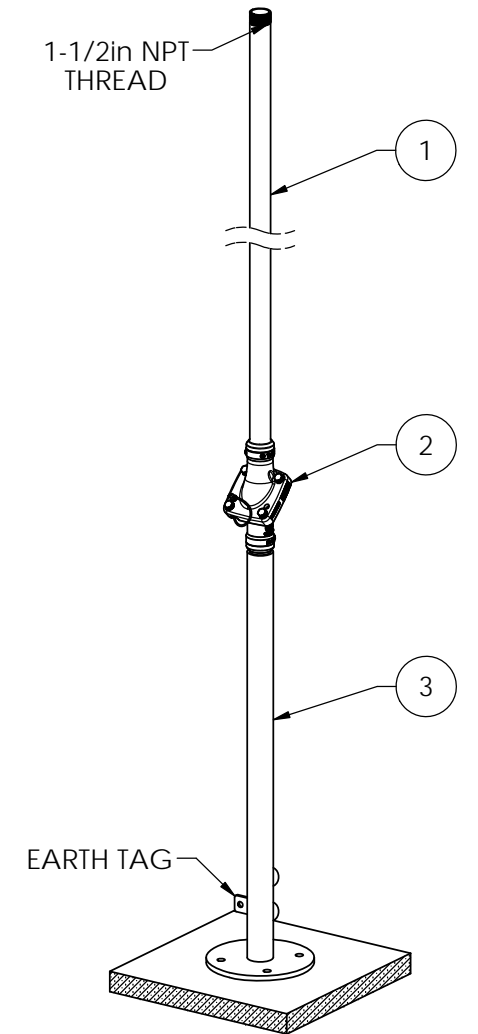
F1-M1 - FLOOR MOUNTED TYPICAL ASSEMBLY
