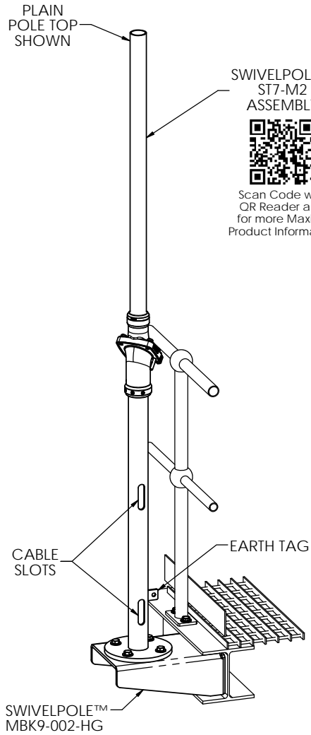
MBK9-002-HG TYPICAL INSTALLATION ALSO SUITS SWIVELPOLE™ ST4-M1 & ST4-M2
